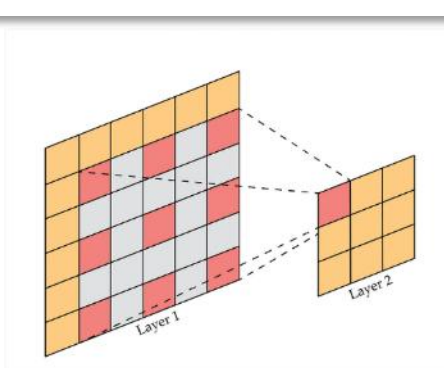
Dilated convolution
